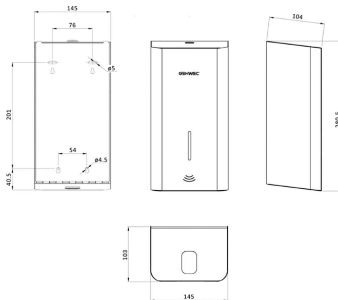
GW04 16 04 03 AISI 304 stainless steel matt black
