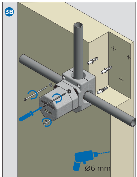
Type 2. Montaje a pared Type 2. Wall mount
